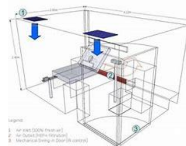
egative Pressure Isolation Ward (Airflow Direction Control)
